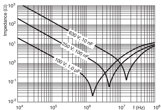
467, 469 - Impedance as a function of frequency (typical curve)
