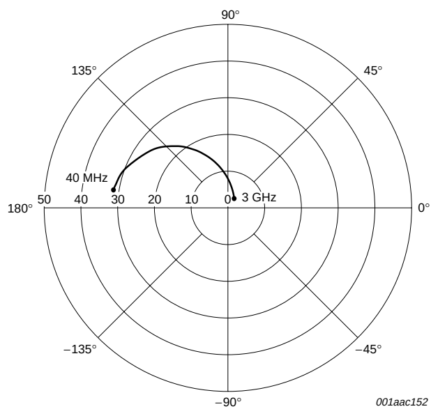
Fig 6. Common emitter forward transmission coefficient ( s_{21} ); typical values
