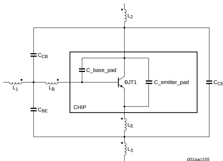
Fig 9. Package equivalent circuit of SOT143R
