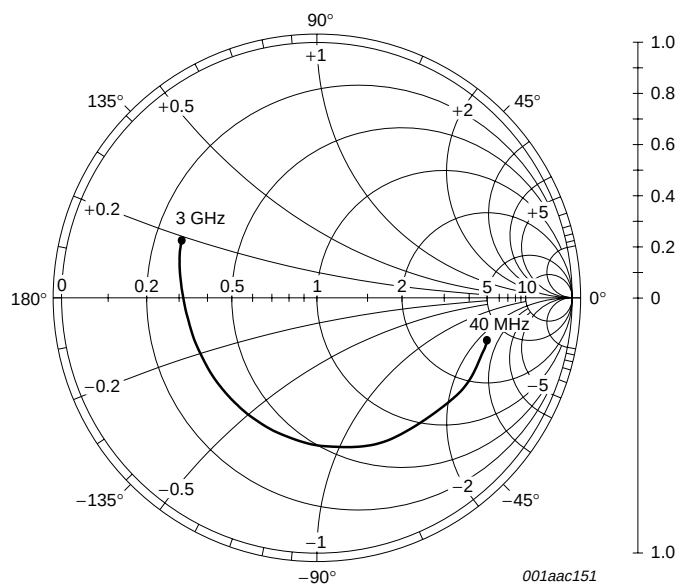
Fig 5. Common emitter input reflection coefficient ( s_{11} ); typical values
