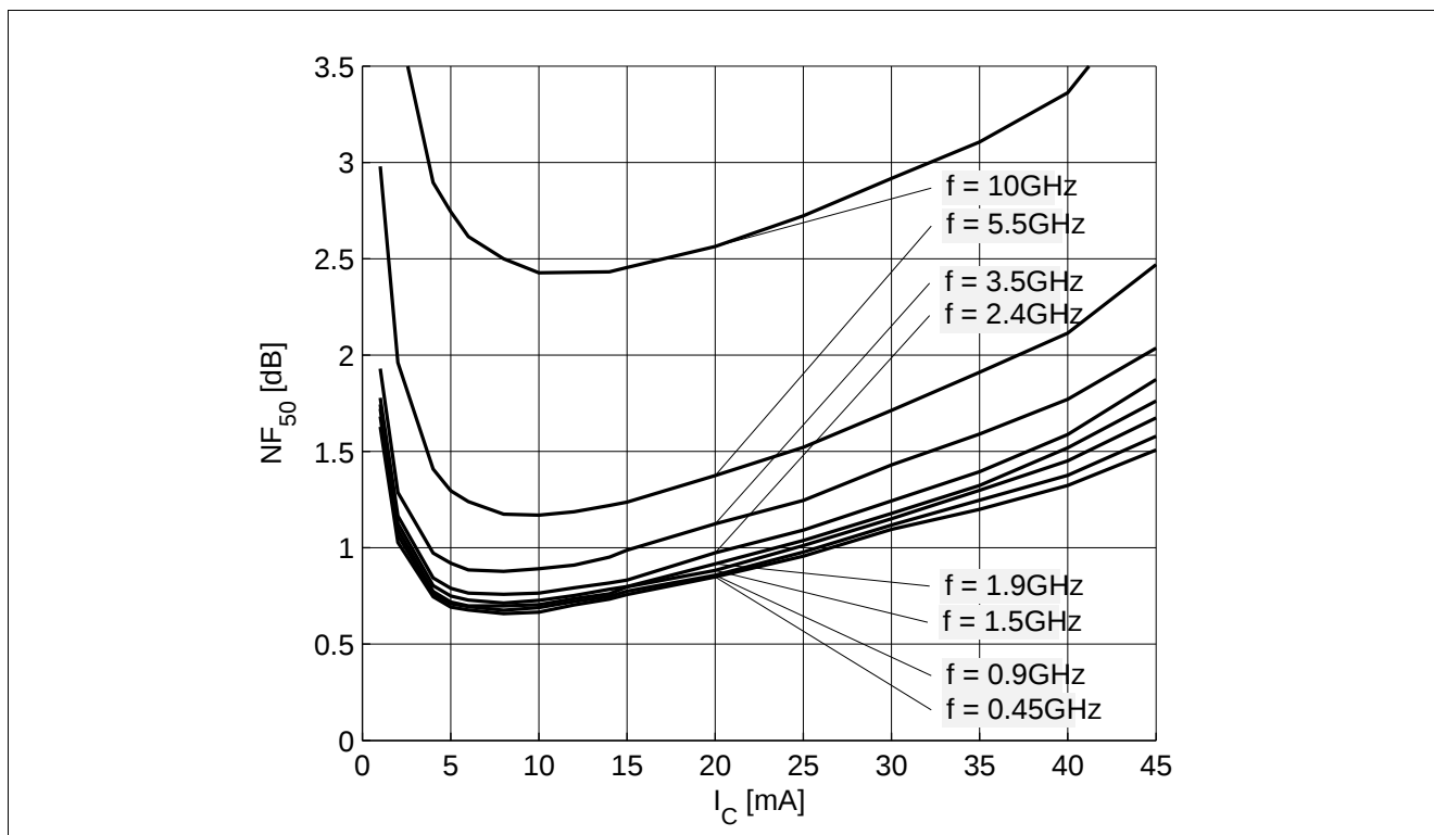
Figure 5-20 Noise Figure NF_{50} = f(I_C) , V_{CE} = 3\text{ V} , Z_S = 50\ \Omega , f = Parameter in GHz
