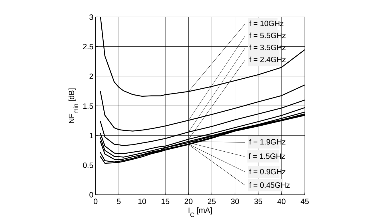
Figure 5-19 Noise Figure NF_{min} = f(I_C) , V_{CE} = 3\text{ V} , Z_S = Z_{opt} , f = Parameter in GHz
