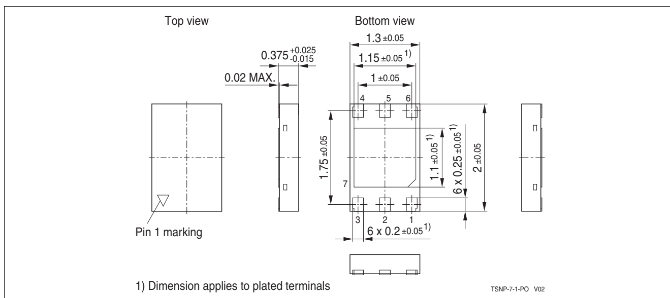
Figure 3 Package Dimensions for TSNP-7-1
