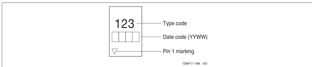
Figure 4 Marking Layout TSNP-7-1 (top view)
