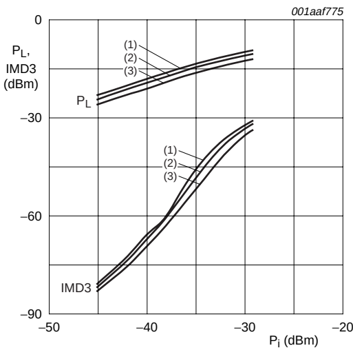
T_{amb} = 25\text{ }^{\circ}\text{C} ; f_1 = 250\text{ MHz} ; f_2 = 251\text{ MHz} ; Z_0 = 50\text{ }\Omega . (1) V_{SUP} = 3.3\text{ V} . (2) V_{SUP} = 3.0\text{ V} . (3) V_{SUP} = 2.7\text{ V} .
