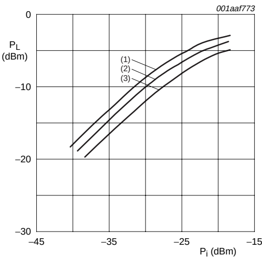
T_{amb} = 25\text{ }^{\circ}\text{C} ; f = 950\text{ MHz} ; Z_0 = 50\text{ }\Omega . (1) V_{SUP} = 3.3\text{ V} . (2) V_{SUP} = 3.0\text{ V} . (3) V_{SUP} = 2.7\text{ V} .
