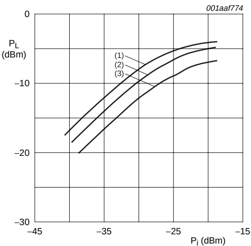
T_{amb} = 25\text{ }^{\circ}\text{C} ; f = 2150\text{ MHz} ; Z_0 = 50\text{ }\Omega . (1) V_{SUP} = 3.3\text{ V} . (2) V_{SUP} = 3.0\text{ V} . (3) V_{SUP} = 2.7\text{ V} .
