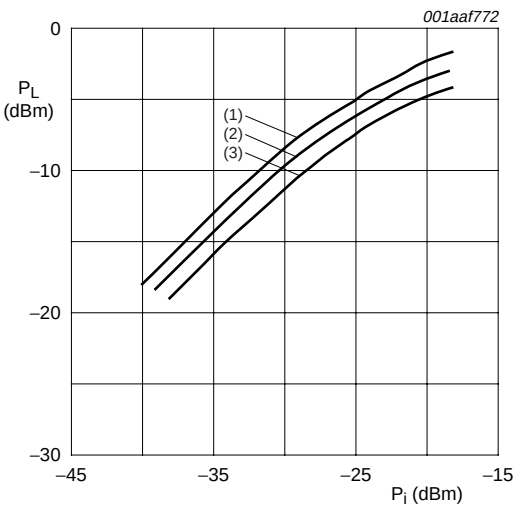
T_{amb} = 25\text{ }^{\circ}\text{C} ; f = 250\text{ MHz} ; Z_0 = 50\text{ }\Omega . (1) V_{SUP} = 3.3\text{ V} . (2) V_{SUP} = 3.0\text{ V} . (3) V_{SUP} = 2.7\text{ V} .
