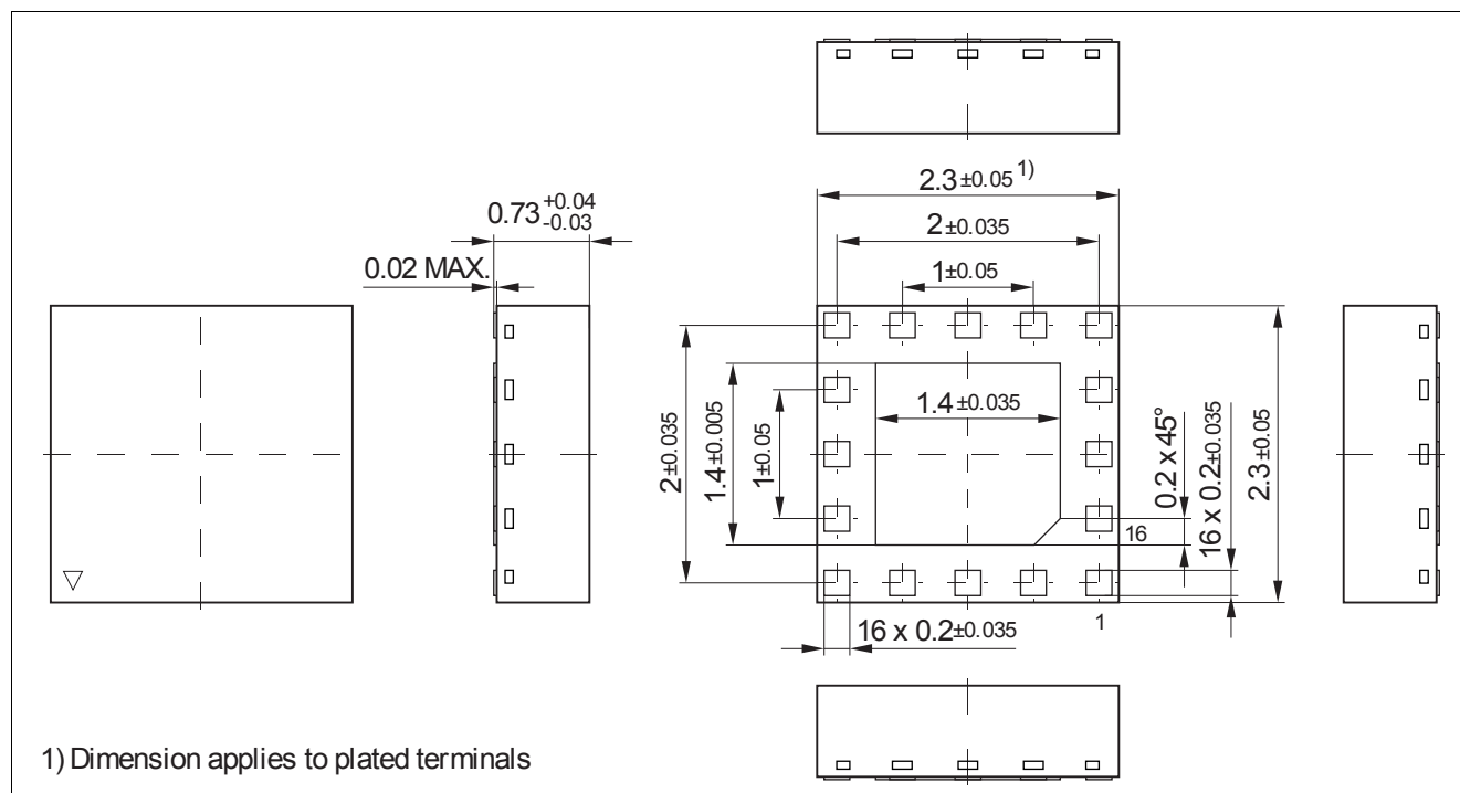
Figure 3 Package Outline
