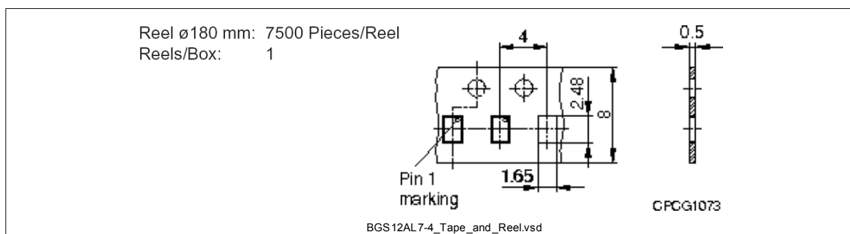
Figure 8 Tape and Reel
