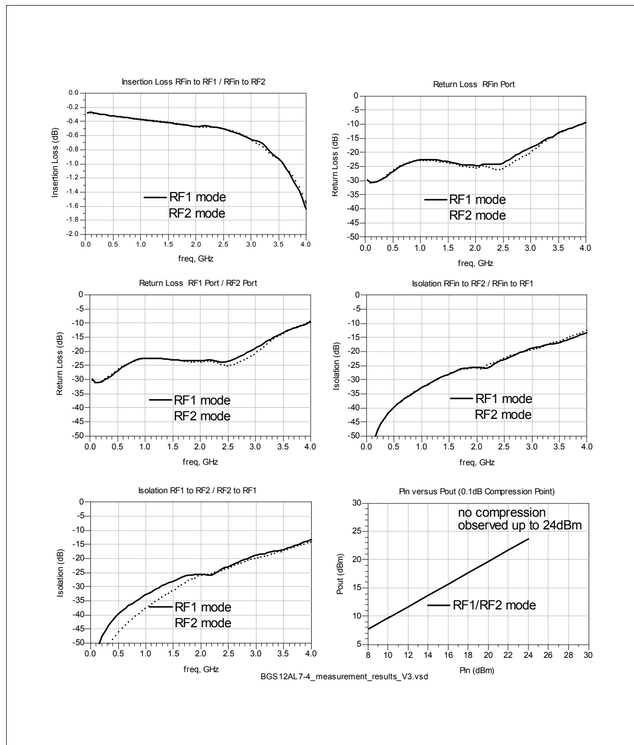
Figure 3 Measurement Results (@ T = 25^{\circ}\text{C} )
