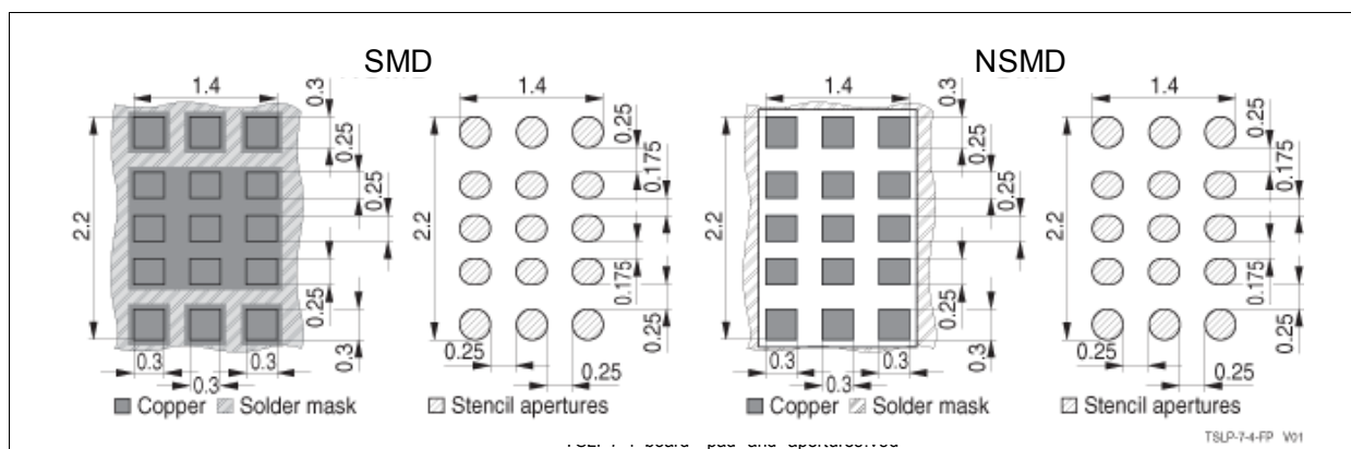
Figure 7 Board Pad (SMD) & Apertures
