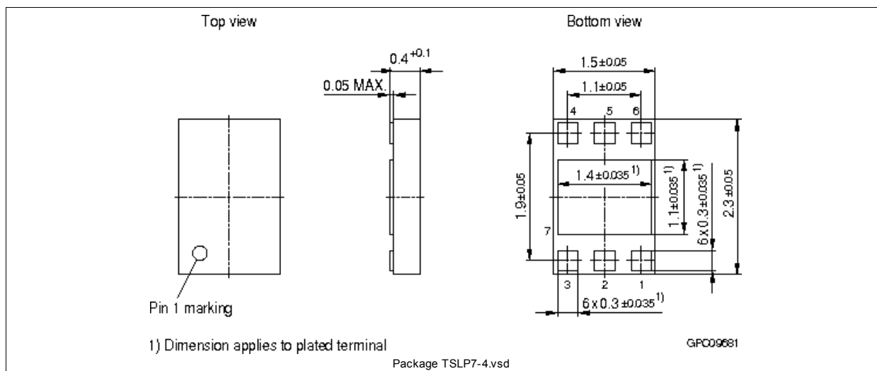
Figure 6 Package TSLP7-4
