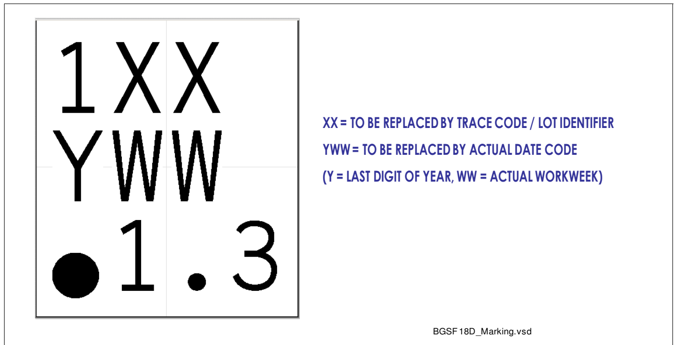
Figure 4 Laser Marking
