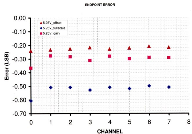
Figure 4. ENDPOINT ERROR vs CHANNEL ( V_{DD}=5.25\text{V} )
