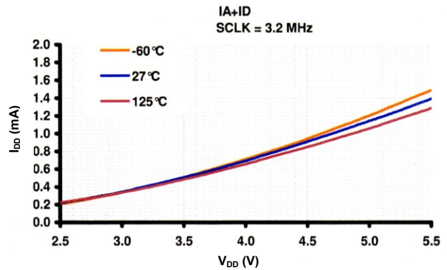
Figure 2. I_{DD} vs V_{DD} ( f_{SCLK}=3.2\text{MHz} )
