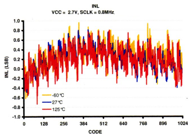
Figure 6. INL vs OUTPUT CODE ( V_{DD}=2.7\text{V} , f_{SCLK}=0.8\text{MHz} , f_{SAMPLE}=50\text{kSPS} )
