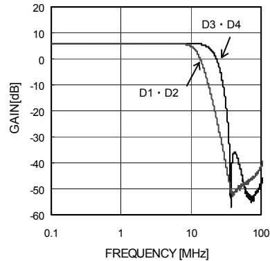
Fig.15 PBLPF Characteristics
