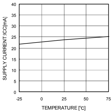
Fig.7 Circuit Current
