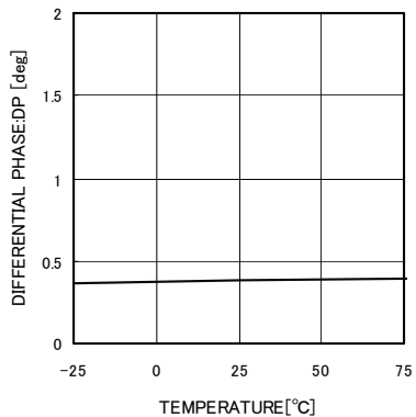
Fig.12 Differential Phase
