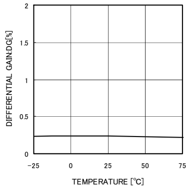
Fig.11 Differential Gain
