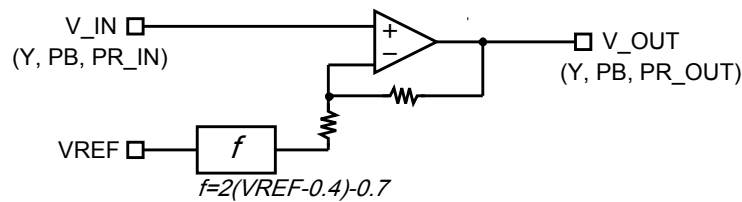
Fig. 3 DC_Shift block equivalent circuit
