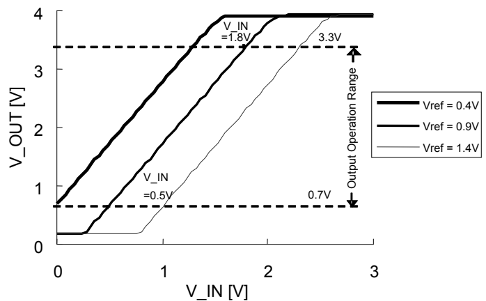
Fig. 5 The relation of V_{IN} - V_{OUT} at each V_{REF} value (measurement value)
