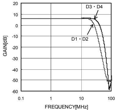
Fig.14 YLPF Characteristics
