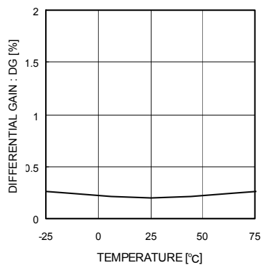
Fig.8 Differential Gain
