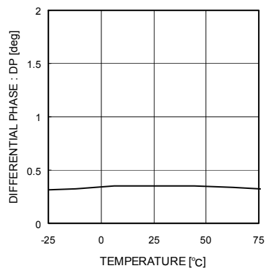
Fig.9 Differential Phase
