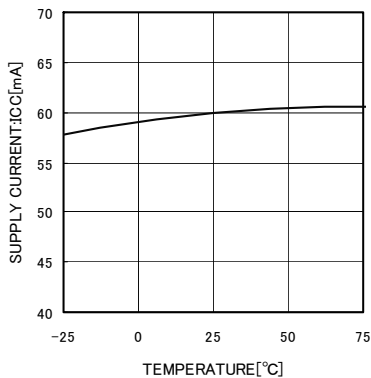
Fig.10 Circuit Current
