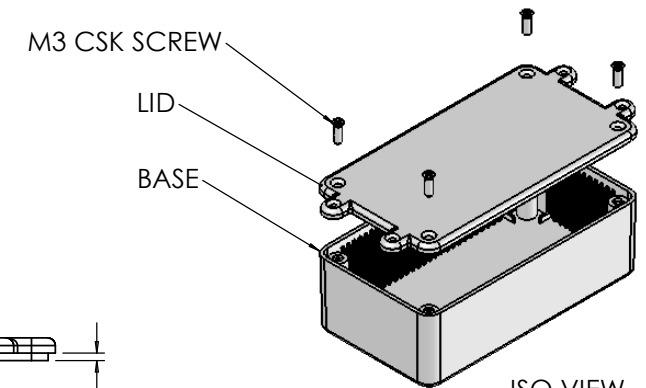
ISO VIEW 1:3
