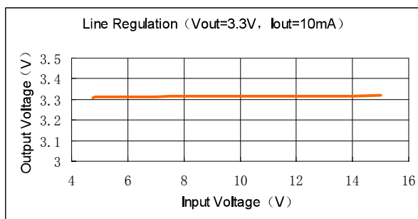
2.BL1117 Line Regulation
