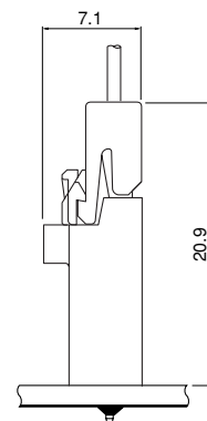
PAF Receptacle + PA high box type header
