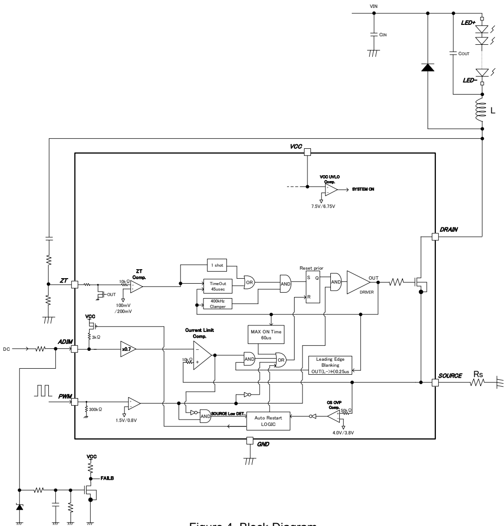
Figure 4. Block Diagram
