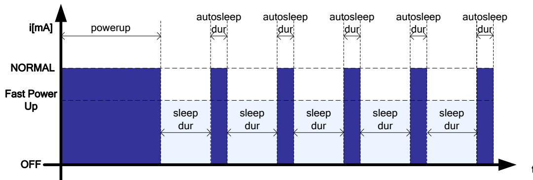
Figure 14: Duty-cycling
