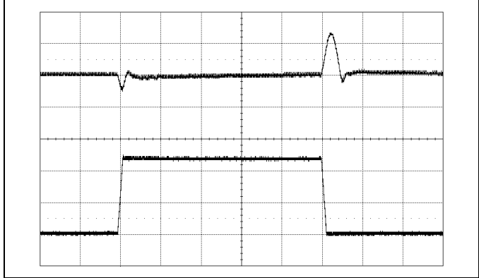
Output Load Transient Response, Default Configuration
