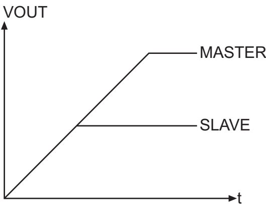
Illustration of Coincident Voltage Tracking.
