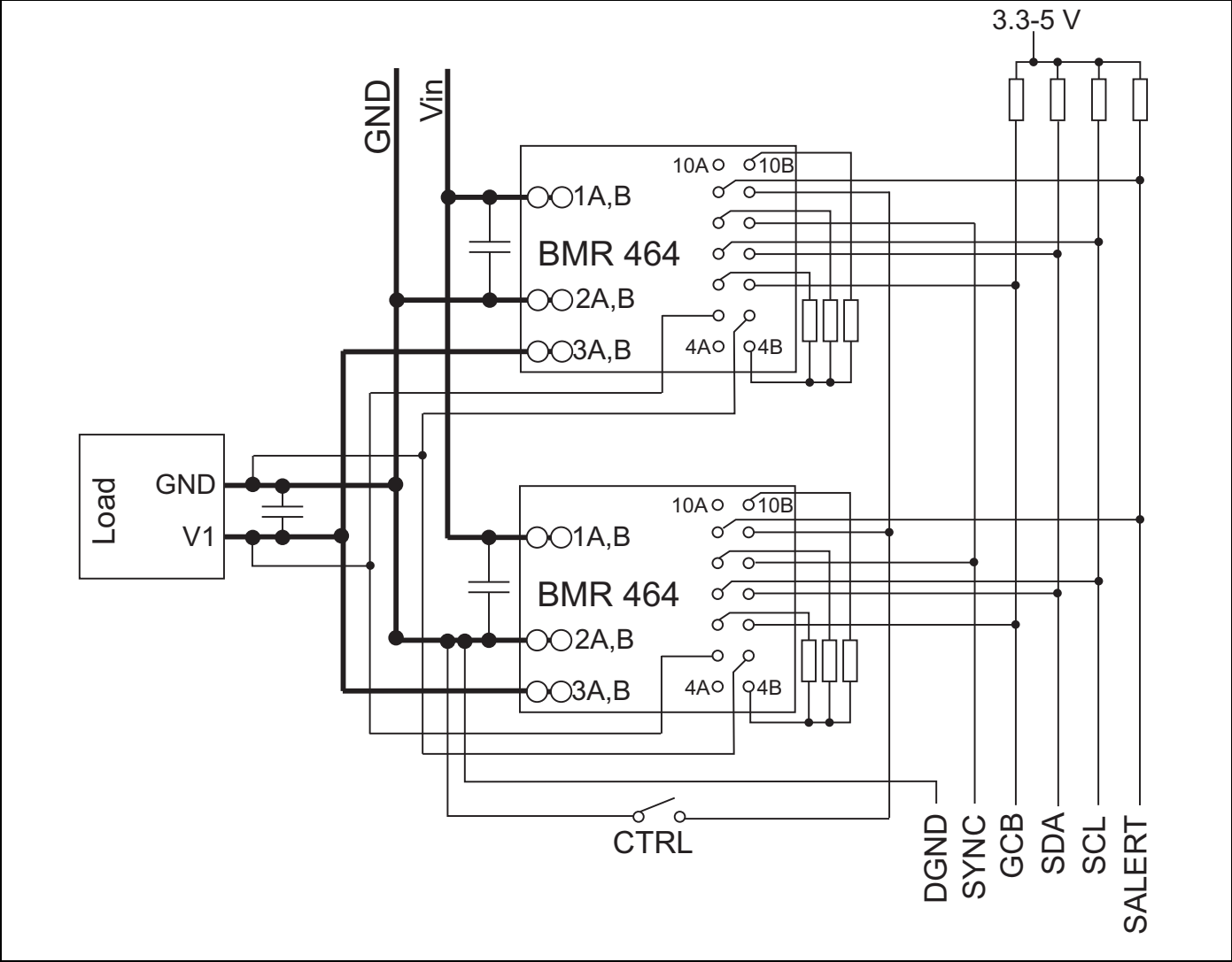
Parallel operation.
