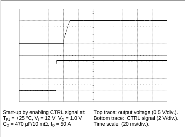
Start-up by CTRL signal
