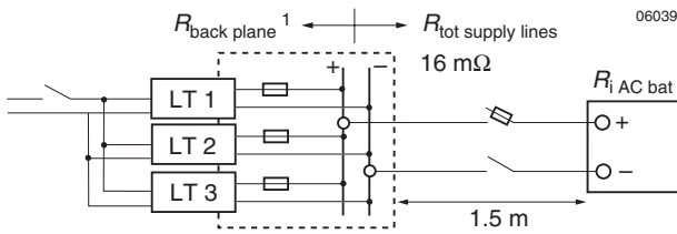
Fig. 10 System set-up
