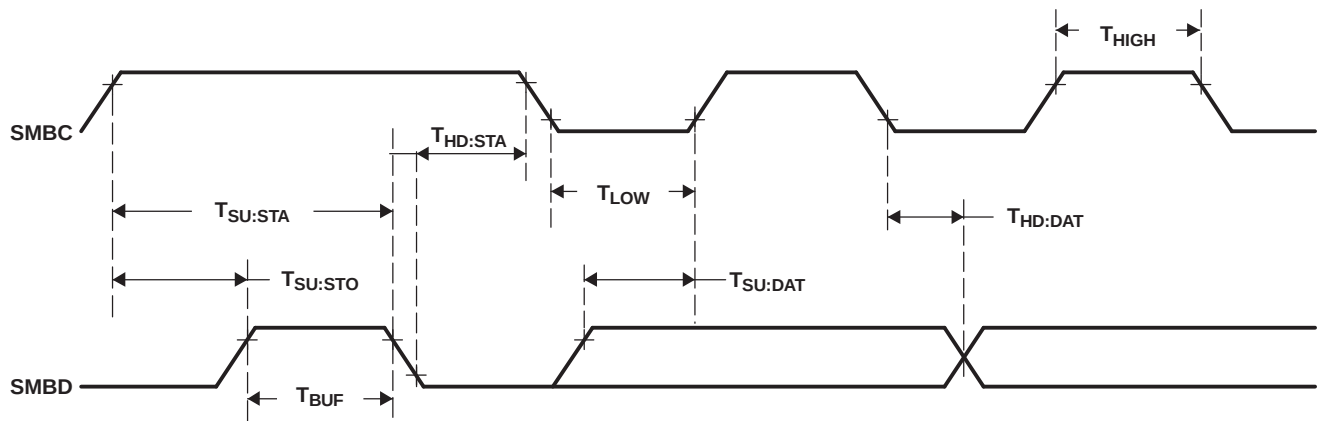
Figure 1. SMBus Timing Data
