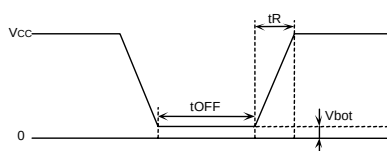
Figure 55. Rise waveform diagram
