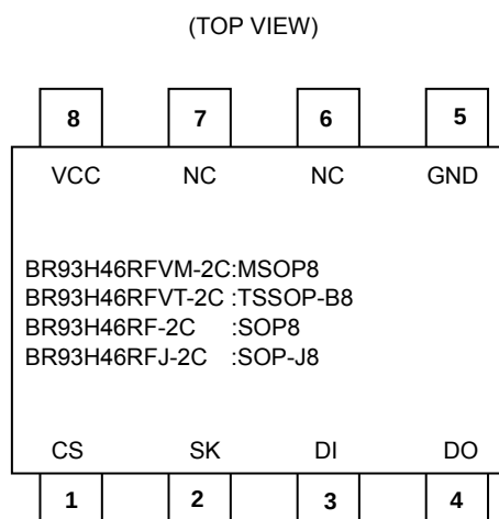
Figure 2. Pin Configuration
