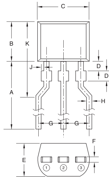
CONNECTION DIAGRAM
