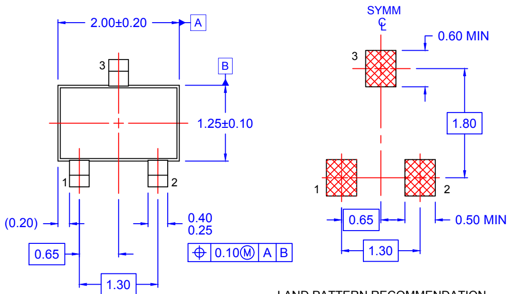
LAND PATTERN RECOMMENDATION
