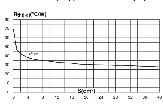
Figure 12. D 2 PAK thermal resistance junction to ambient versus copper surface under tab (printed circuit board FR4, copper thickness: 35 \mu\text{m} )
