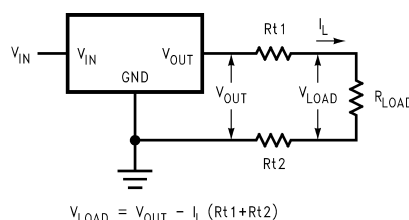
Figure 7. Typical Application using Fixed Output Regulator
