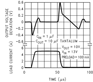
LM1084-ADJ Load Transient Response
