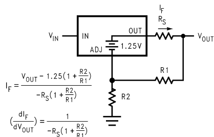
Figure 16. Battery Charger
