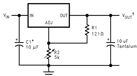
Figure 4. 1.2V to 15V Adjustable Regulator
