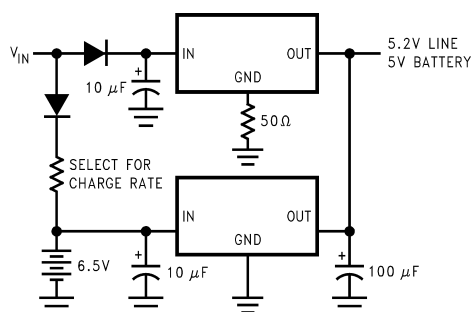
Figure 20. Battery Backup Regulated Supply
