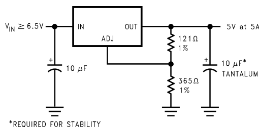
Figure 13. Adjustable @ 5V
