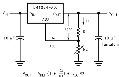
Figure 6. Basic Adjustable Regulator
