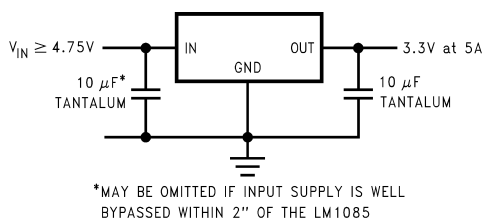
Figure 12. 5V to 3.3V, 5A Regulator
