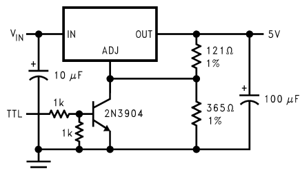
Figure 13. Adjustable @ 5V
