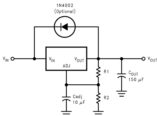
Figure 9. Regulator with Protection Diode
