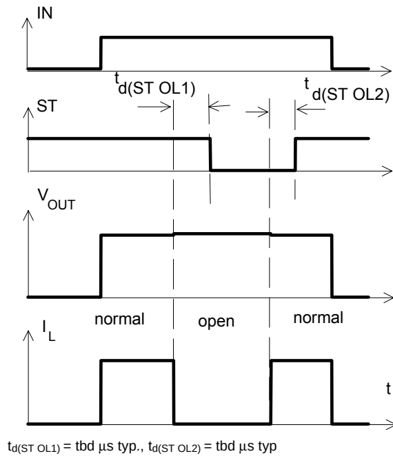
Figure 6a: Undervoltage:
