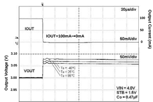
Fig 222. Load Response
