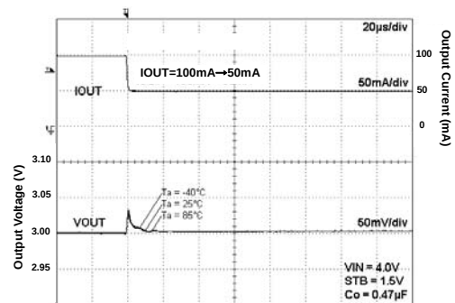
Fig 226. Load Response
