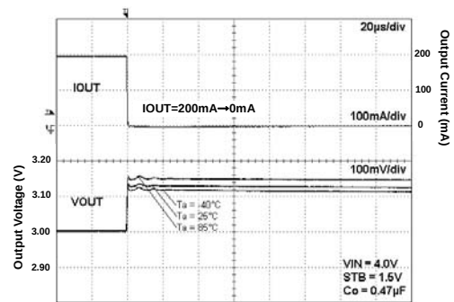
Fig 224. Load Response
