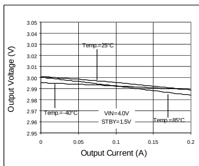
Fig. 127 Load Regulation
