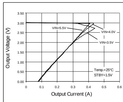
Fig. 128 OCP Threshold
