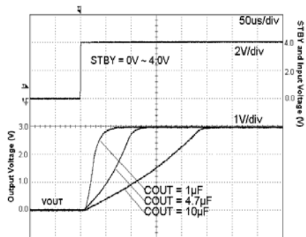
Fig. 147 Start Up Time (STBY=VIN) I_{out} = 200\text{mA}
