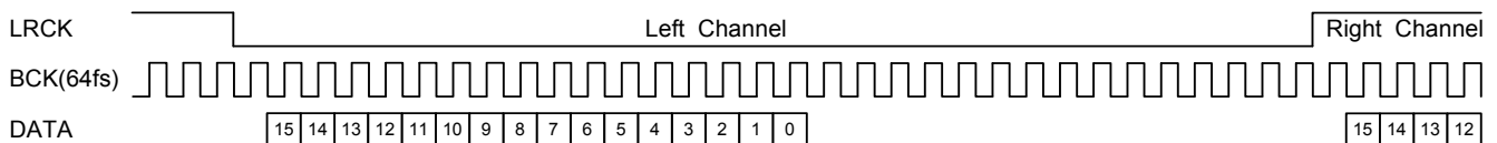
Figure 5.6.3 I 2 S Output Timing (64fs)
