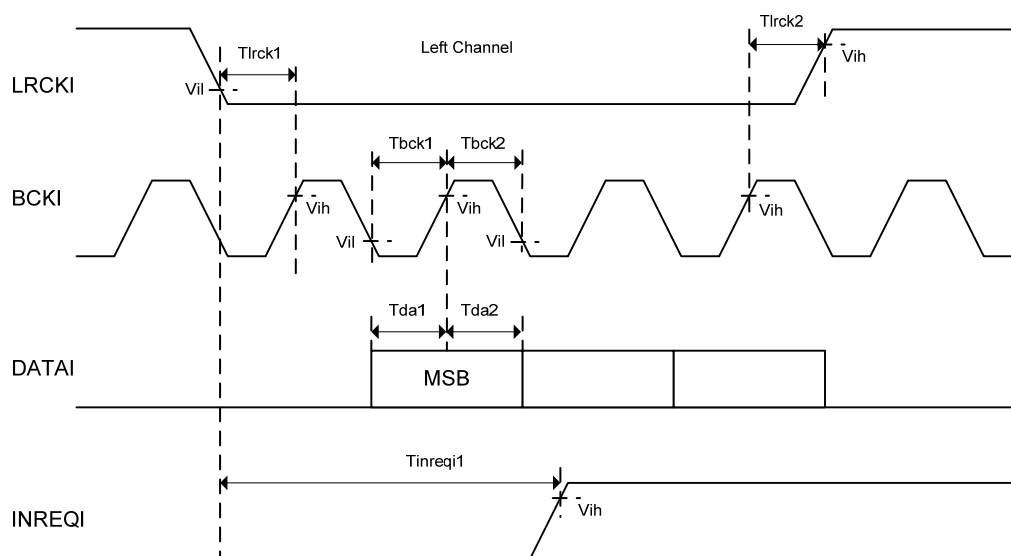
Figure 5.13.2 CD I/F Timing
