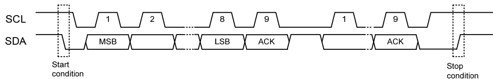
Figure 5.8.1 I 2 C Start and Stop Conditions
