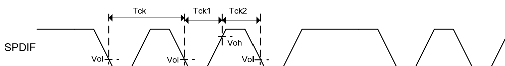
Figure 5.7.2 SPDIF Output Timing
