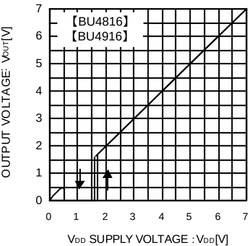
Fig.6 I/O Characteristics
