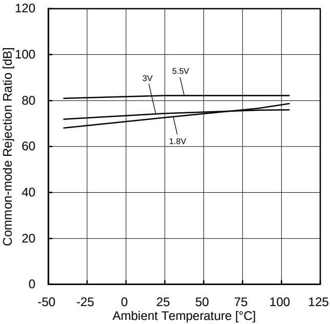
Figure 19. Common-mode Rejection Ratio vs Ambient Temperature (VDD=3V)
