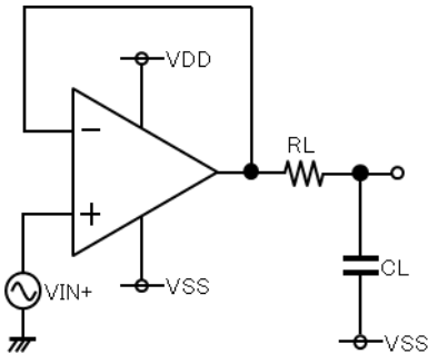
Figure 38. Improvement circuit example 1
