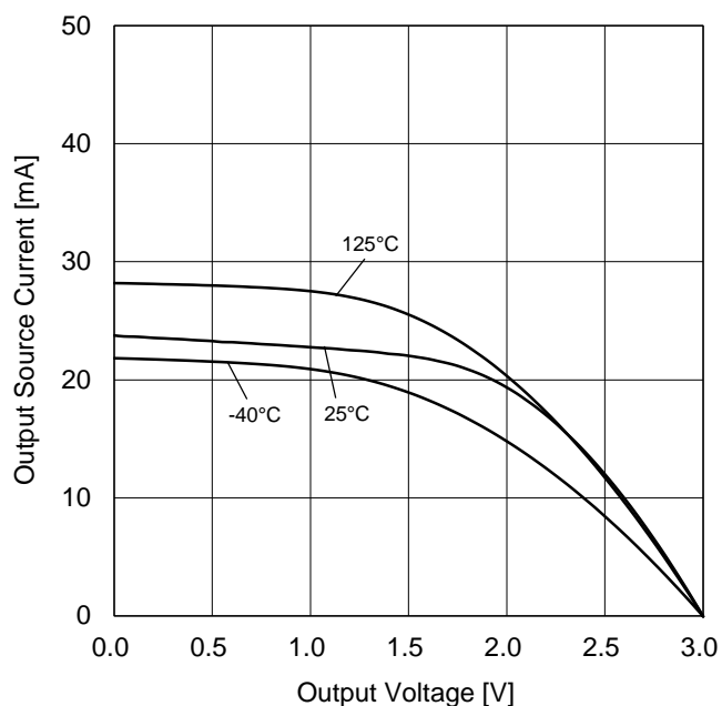
Figure 10. Output Source Current vs Output Voltage (VDD=3.0V)
