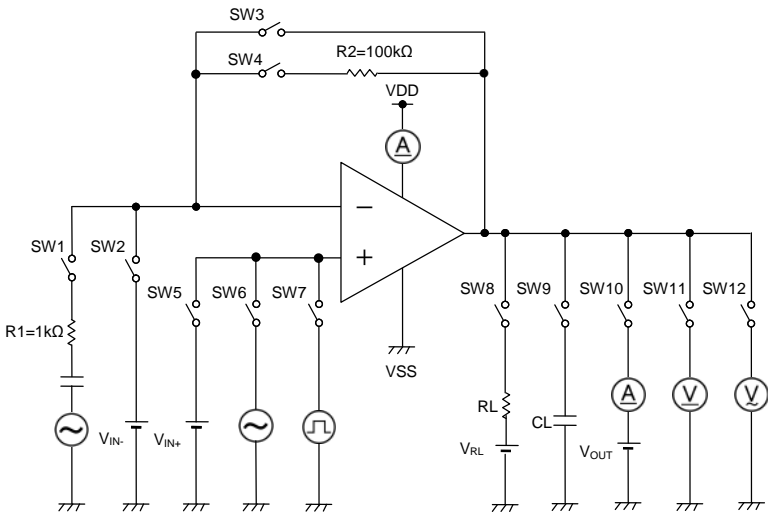
Figure 31. Test Circuit 2
