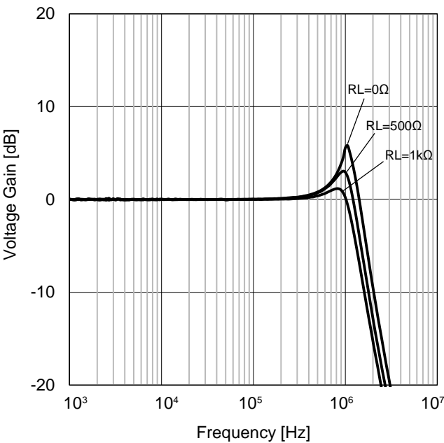
Figure 40. Voltage Gain vs Frequency (VDD=3.0V,Gv=0dB,CL=100pF,Circuit:Figure38)
