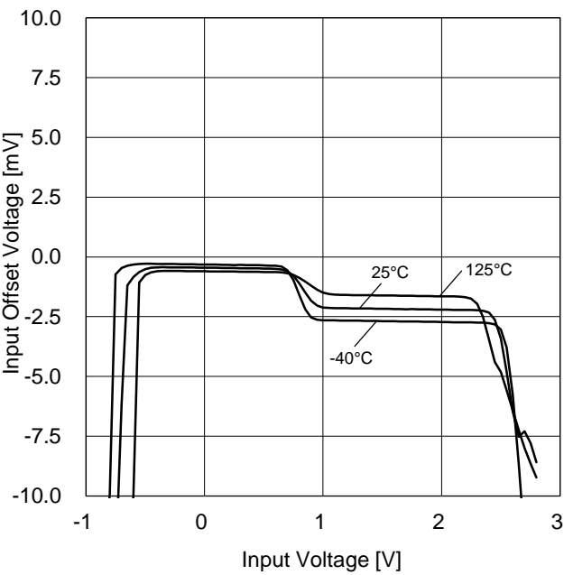
Figure 19. Input Offset Voltage vs Input Voltage ( V_{DD}=1.8V )
