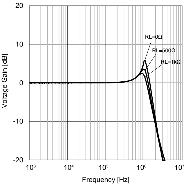
Figure 41. Voltage Gain vs Frequency (VDD=3.0V,Gv=0dB,CL=100pF,Circuit:Figure39)
