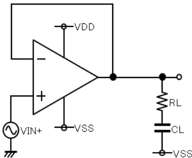
Figure 39. Improvement circuit example 2
