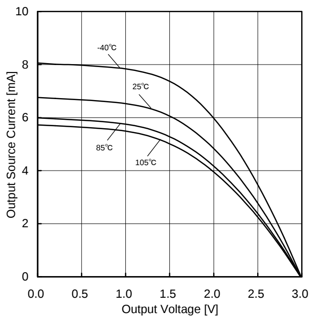
Figure 10. Output Source Current vs Output Voltage (VDD=3V)
