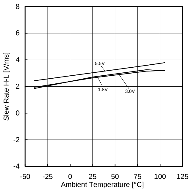
Figure 46. Slew Rate H-L vs Ambient Temperature
