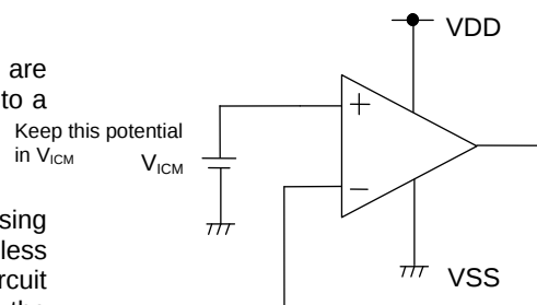
Figure 58. Example of Application Circuit for Unused Op-amp
