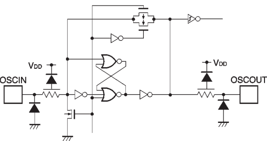
Fig. 13 Oscillation circuit
