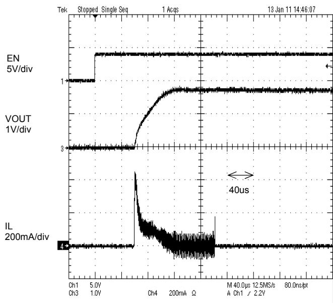
Figure 28. Start up
