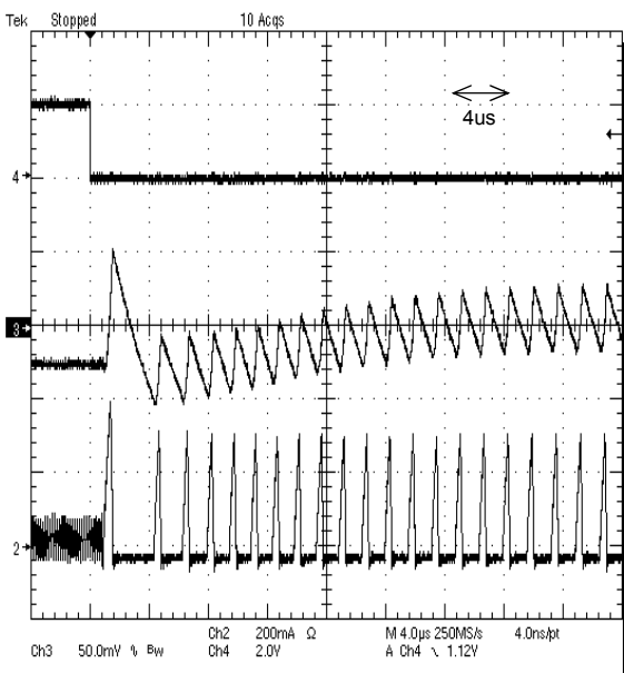
Figure 46. Mode Change Response MODE : High to Low
