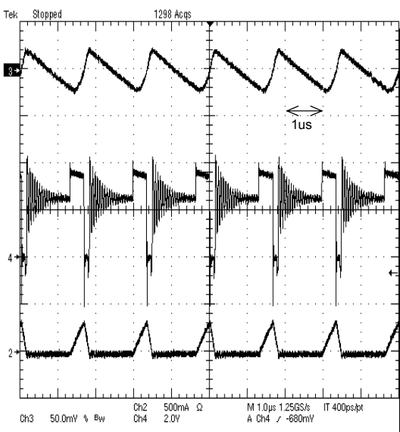
Figure 44. PFM mode Operation Iout=50mA
