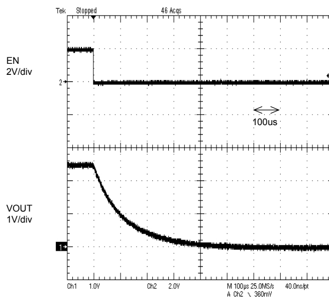
Figure 40. Shut down
