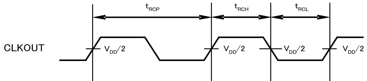
Figure 7. CLKOUT Period and High/Low Time
