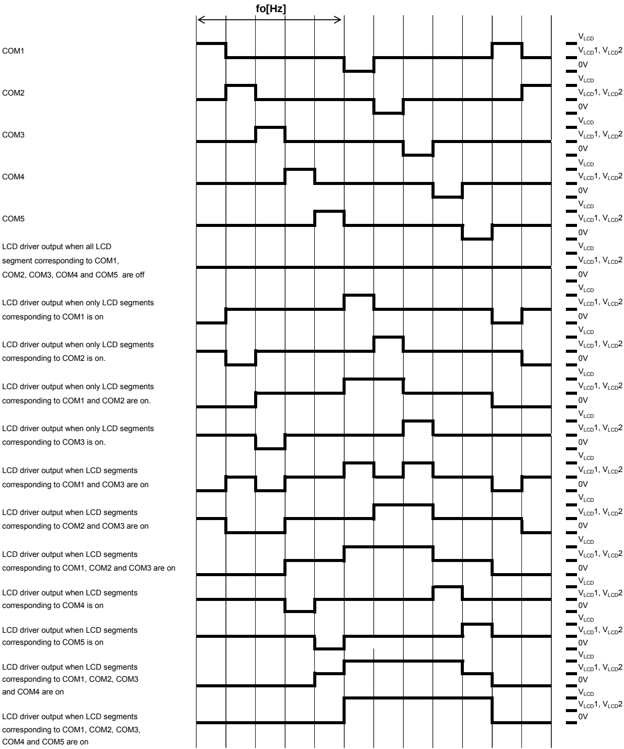
Figure 32. LCD Waveform (Frame Inversion, 1/5 DUTY, 1/2BIAS)
