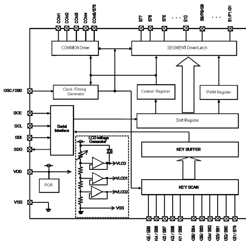
Figure 2. Block Diagram
