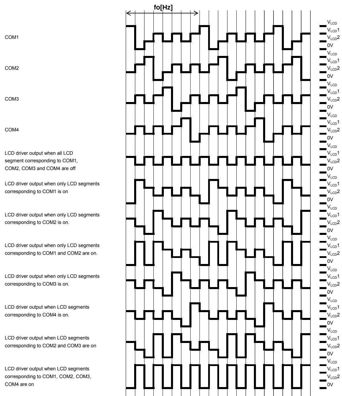
Figure 26. LCD Waveform (Line Inversion, 1/4 DUTY, 1/3 BIAS)
