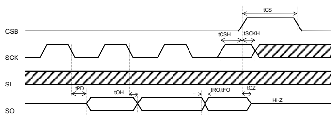
Fig.2 Input and output timing
