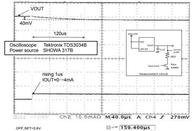
BU9829GUL-W Evaluation result ( I_{OUT}=0\text{mA}\rightarrow 4\text{mA} , C_{OUT}=1.0\mu\text{F} ) Fig.59 C_L=10\mu\text{F} Transitional response
