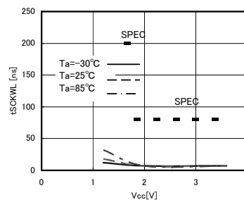
Fig.18 SCK low time t_{SCKWL}
