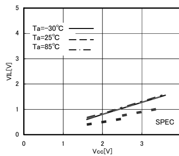
Fig.8 "L" input voltage VIL (EEPROM)
