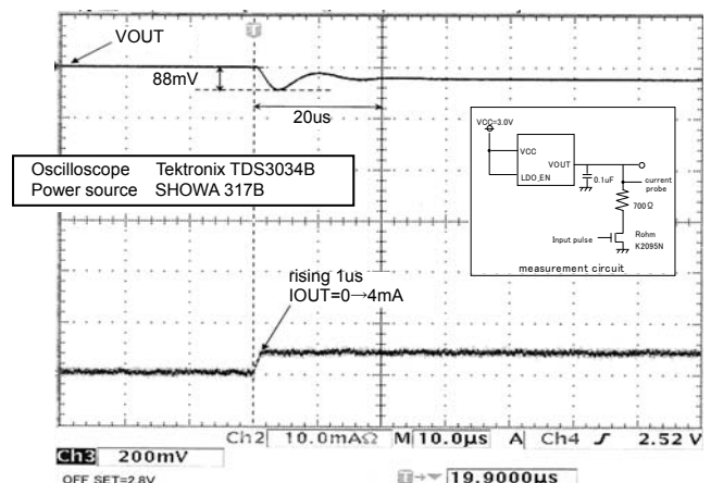
BU9829GUL-W Evaluation result ( I_{OUT}=0\text{mA}\rightarrow 4\text{mA} , C_{OUT}=0.1\mu\text{F} ) Fig.57 C_L=0.1\mu\text{F} Transitional response
