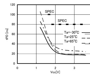
Fig.24 Data output delay time t_{PD}
