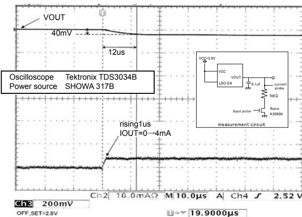
BU9829GUL-W Evaluation result ( I_{OUT}=0\text{mA}\rightarrow 4\text{mA} , C_{OUT}=1.0\mu\text{F} ) Fig.58 C_L=1.0\mu\text{F} Transitional response
