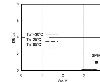
Fig.27 Standby operation ISB (LDO)
