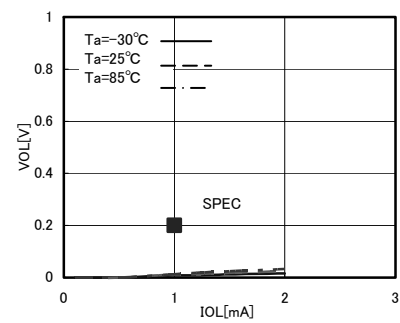
Fig.9 "L" output voltage VOL
