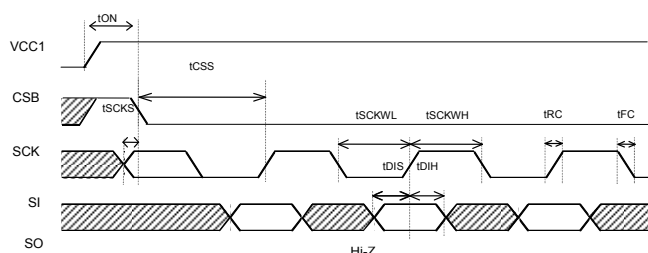
Fig.1 Input timing
