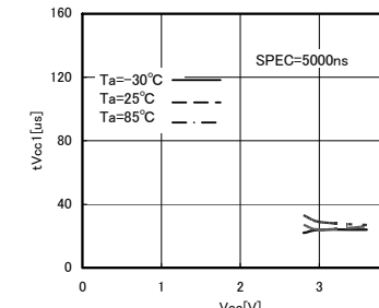
Fig.30 V_{CC1} rise time t_{Vcc1}
