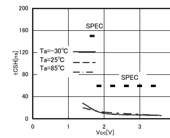
Fig.21 CSB hold time t_{CSH}
