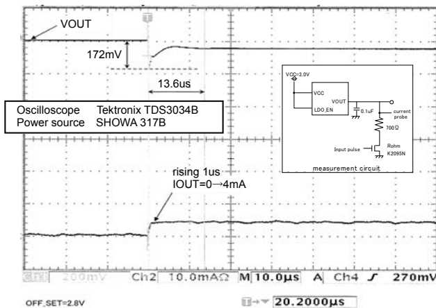
BU9829GUL-W Evaluation result ( I_{OUT}=0\text{mA}\rightarrow 4\text{mA} , C_{OUT}=1.0\mu\text{F} ) Fig.56 C_L=0\mu\text{F} Transitional response
