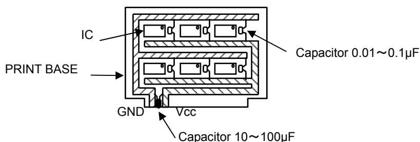
Fig.63 Vcc noise countermeasures example
