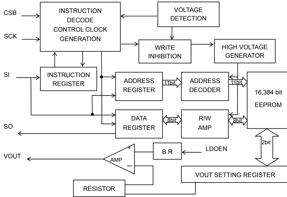
Fig.6 Block diagram
