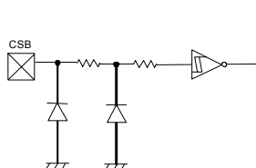
Fig.47 CSB terminals equivalent circuit
