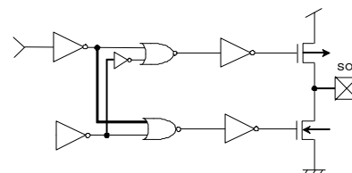
Fig.49 SO terminals equivalent circuit
