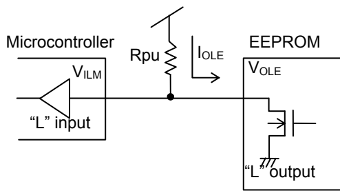
Fig.52 SO Pull up resistance
