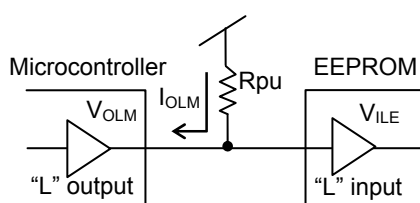
Fig.50 Input terminal pull up resistance
