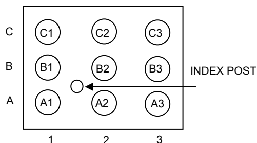
Fig.3 Pin configuration (bottom view)
