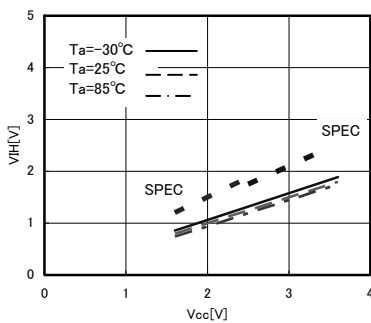
Fig.7 "H" input voltage VIH (EEPROM)
