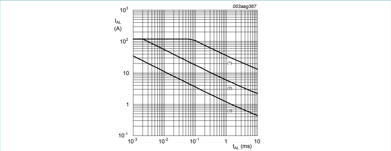
Fig. 4. Avalanche rating; avalanche current as a function of avalanche time. (1) T_{j(init)} = 25^{\circ}C ; (2) T_{j(init)} = 150^{\circ}C ; (3) Repetitive Avalanche
