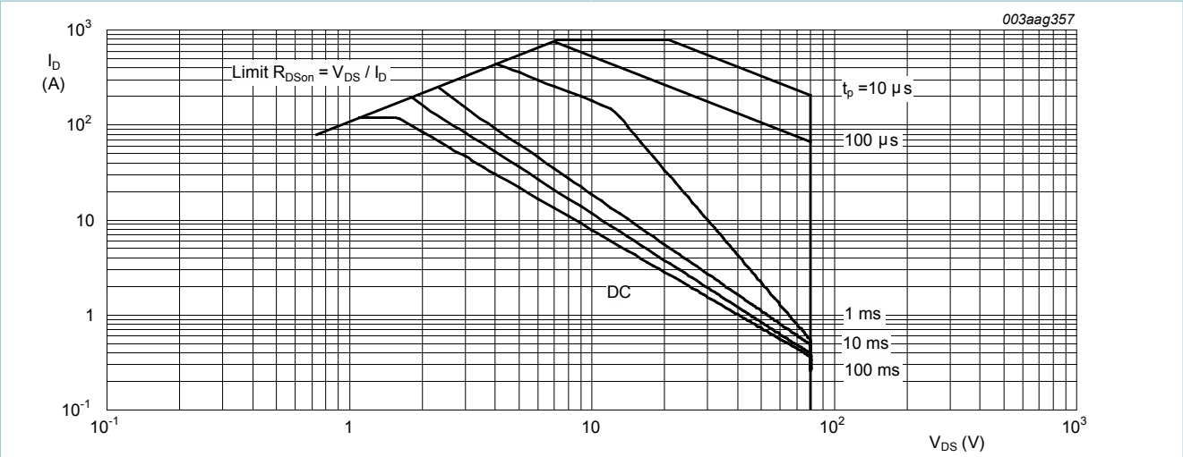
Fig. 3. Safe operating area; continuous and peak drain currents as a function of drain-source voltage T_{mb} = 25^{\circ}C ; I_{DM} is a single pulse
