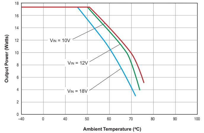
BWR-12/725-D12A Output Power vs. Ambient Temperature (No air flow)
