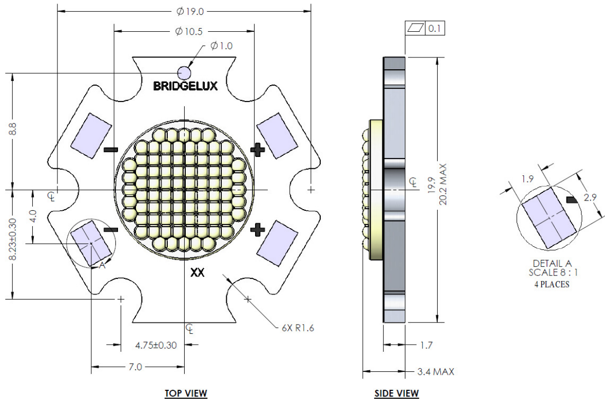
Figure 1: Drawing for all BXRB ES Star Arrays.
