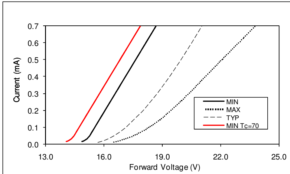
Figure 10: Typical Current vs. Voltage, BXR-XXX0540-A, BXR-56C0700-A
