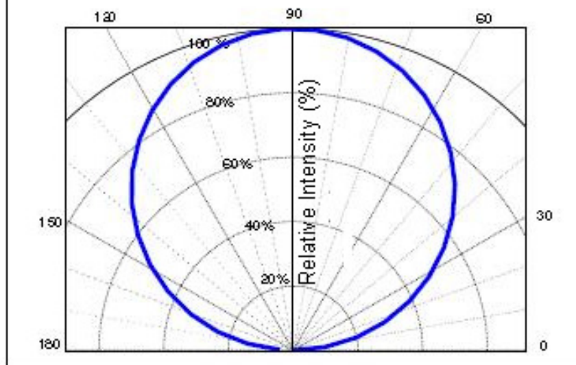
Figure 3: Typical Far Field Polar Radiation Pattern
