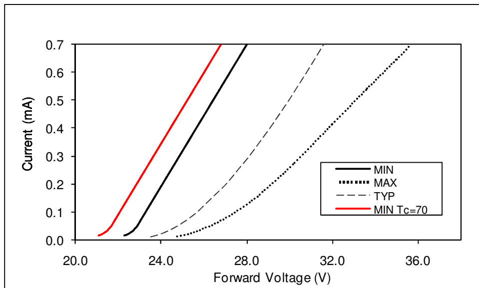
Figure 11: Typical Current vs. Voltage BXR-XXX0740-A, BXR-40E0810-A, BXR-56C1000
