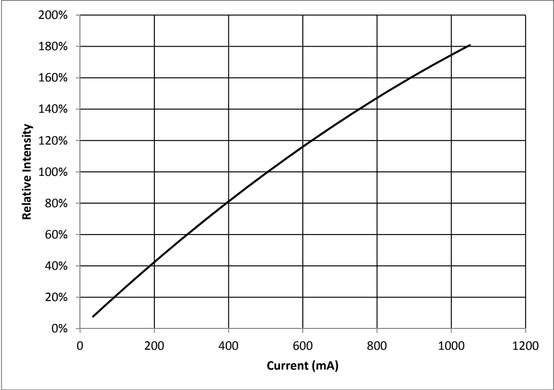
Figure 2: Typical Flux vs. Current, Tj = 25°C
