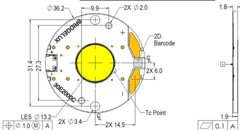
Figure 9: Drawing for Vero 13 LED Array
