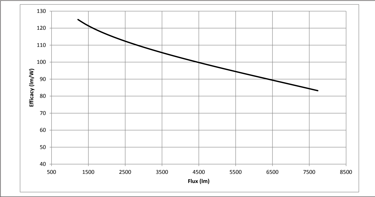
Figure 2: Efficacy vs. Flux ( T_j = T_c = 25^{\circ}\text{C} ; BXRH-30E6000-G-23)
