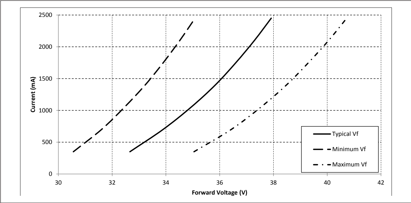
Figure 3: Drive Current vs. Voltage ( T_j = T_c = 25^{\circ}\text{C} )
