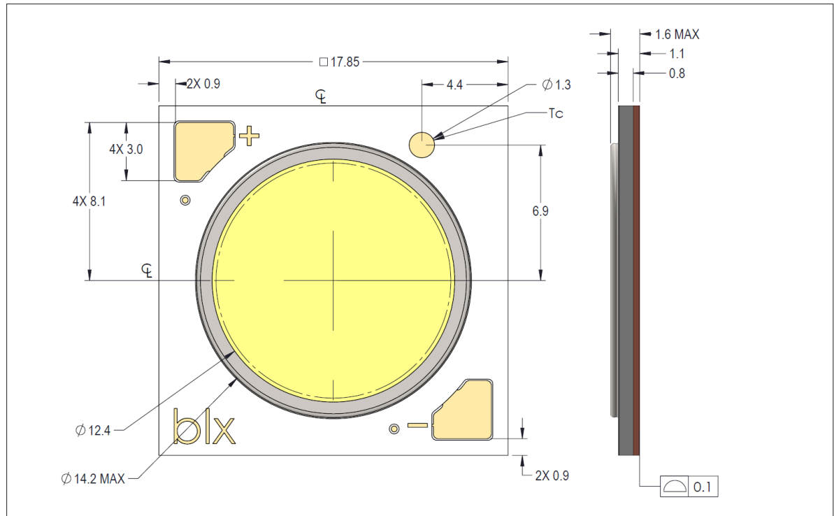
Figure 10: Drawing for H12 LED Array
