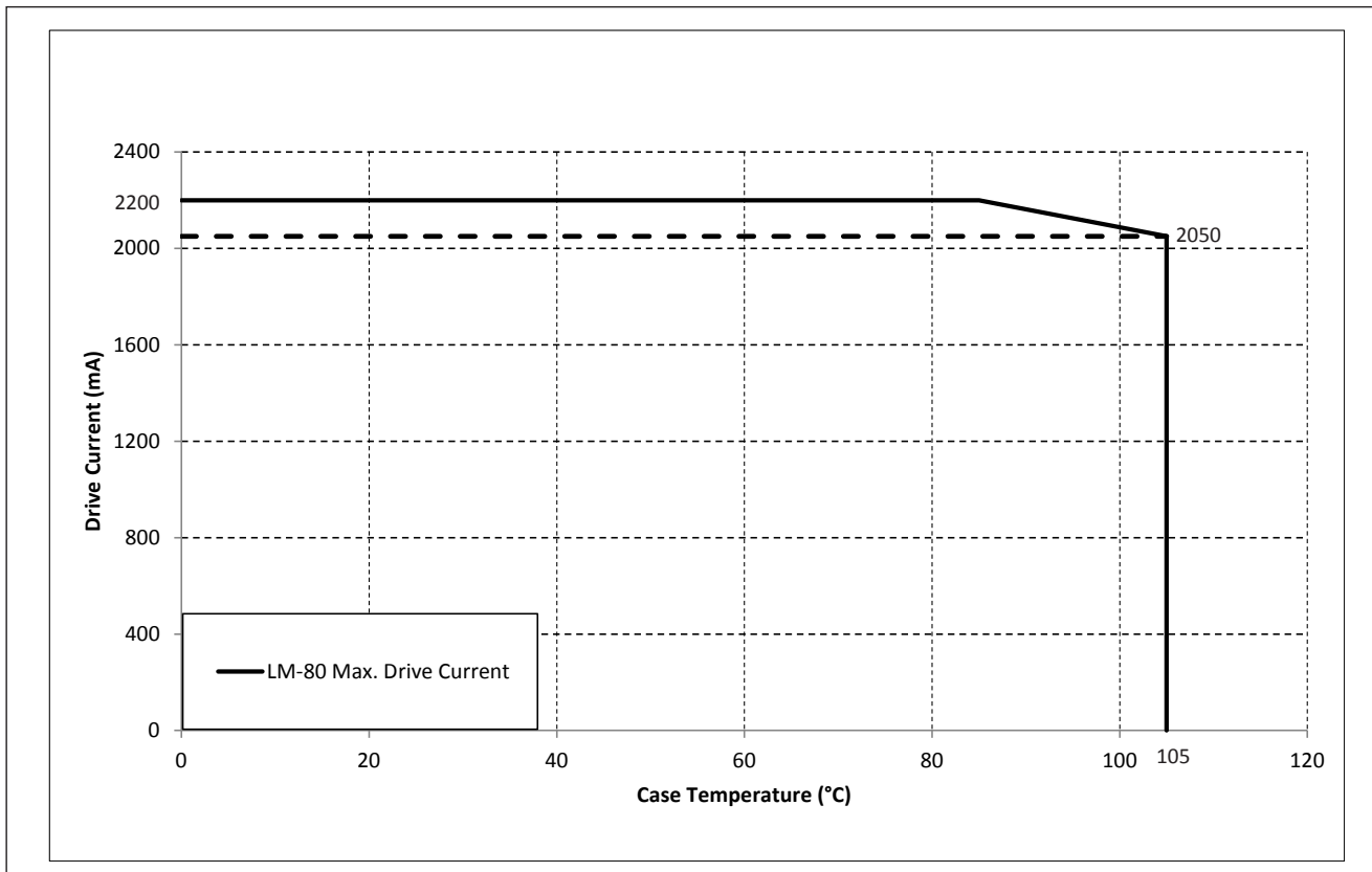
Figure 1: H12 Drive Current Derating Curve ( T_j = T_c = 25^\circ\text{C} )
