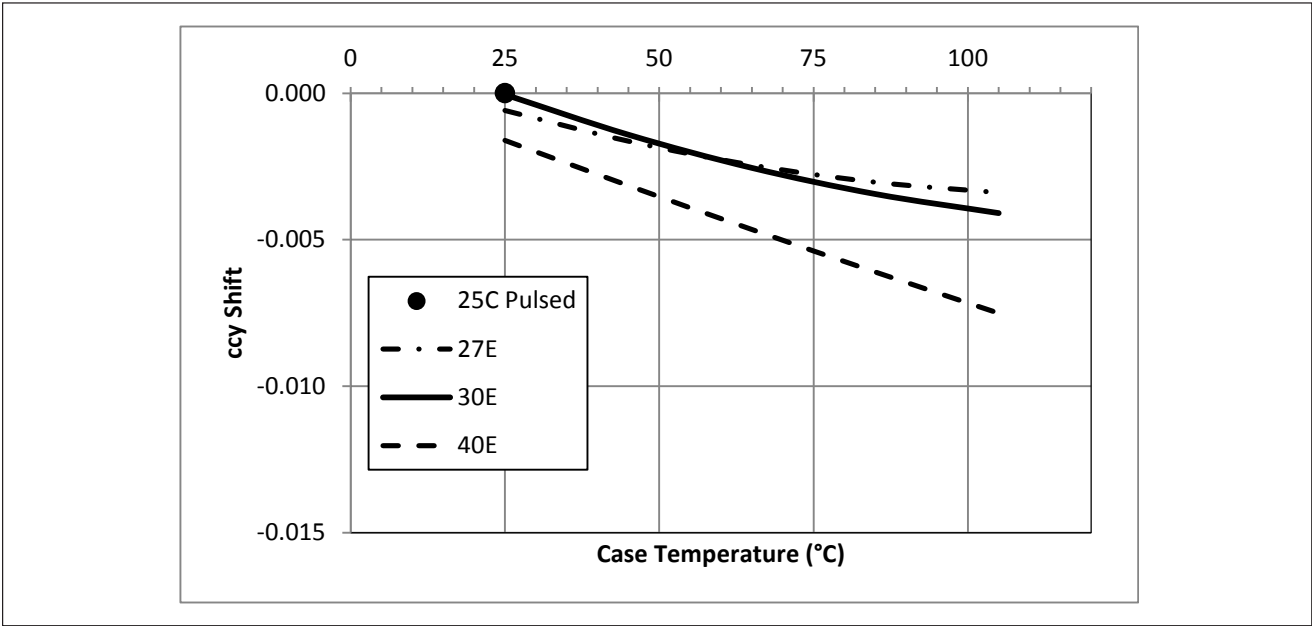
Figure 6: Typical DC ccy Shift vs. Case Temperature
