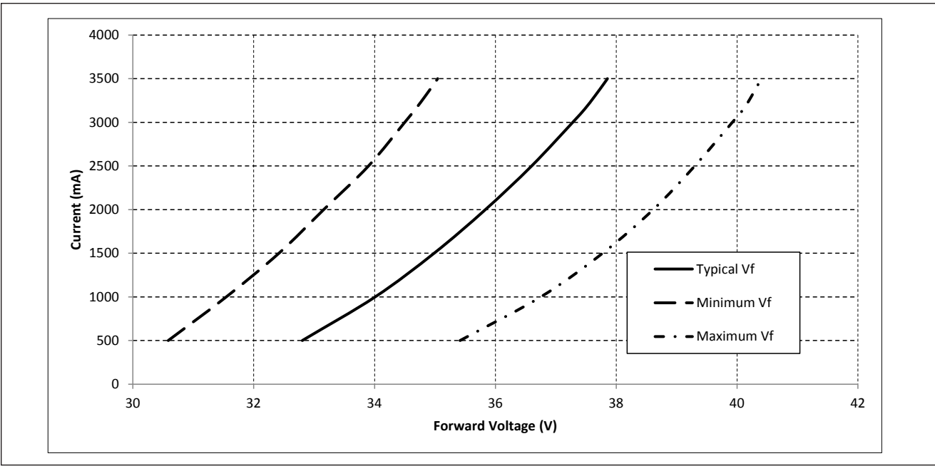
Figure 2: Drive Current vs. Voltage ( T_j = T_c = 25^{\circ}\text{C} )
