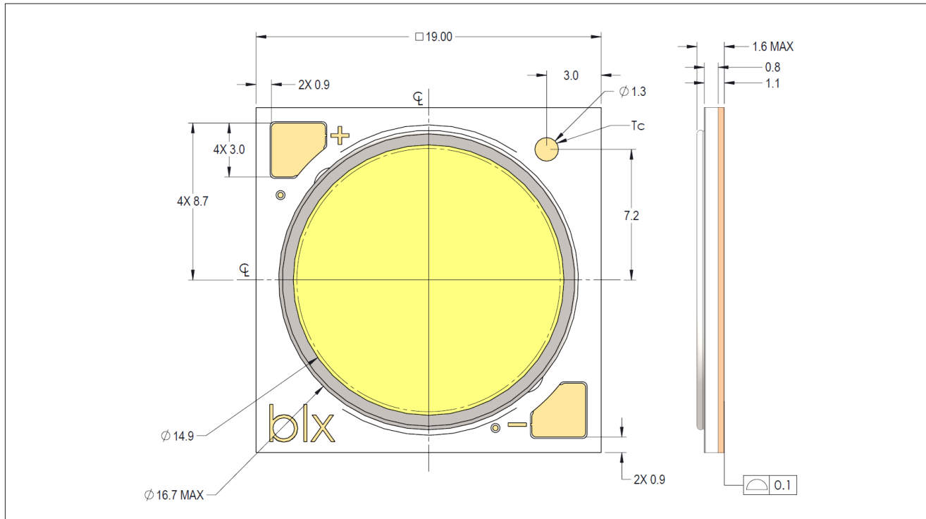
Figure 9: Drawing for H15 LED Array
