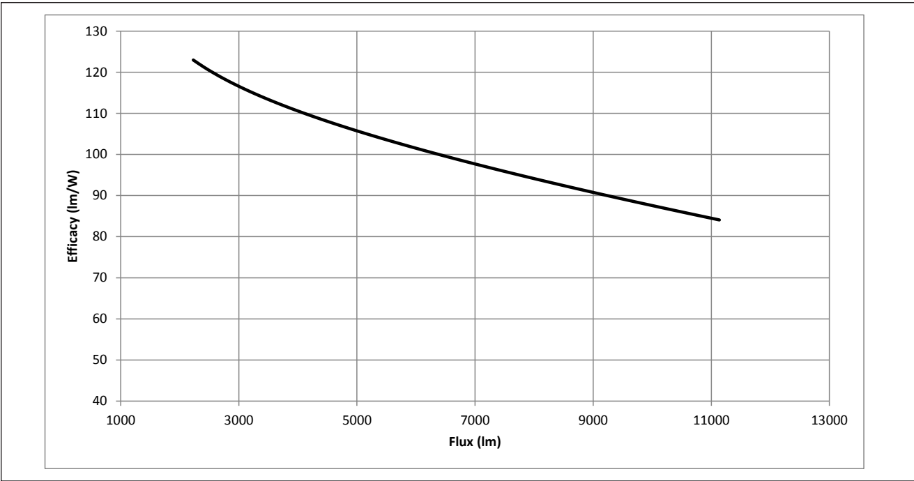
Figure 1: Efficacy vs. Flux ( T_j = T_c = 25^{\circ}\text{C} ; BXRH-30E8000-J-23)
