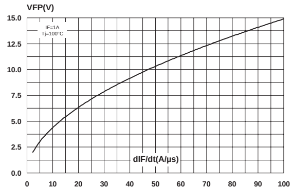
Fig. 8: Transient peak forward voltage versus dI_F/dt (90% confidence).
