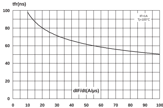
Fig. 7: Forward recovery time versus dI_F/dt (90% confidence).
