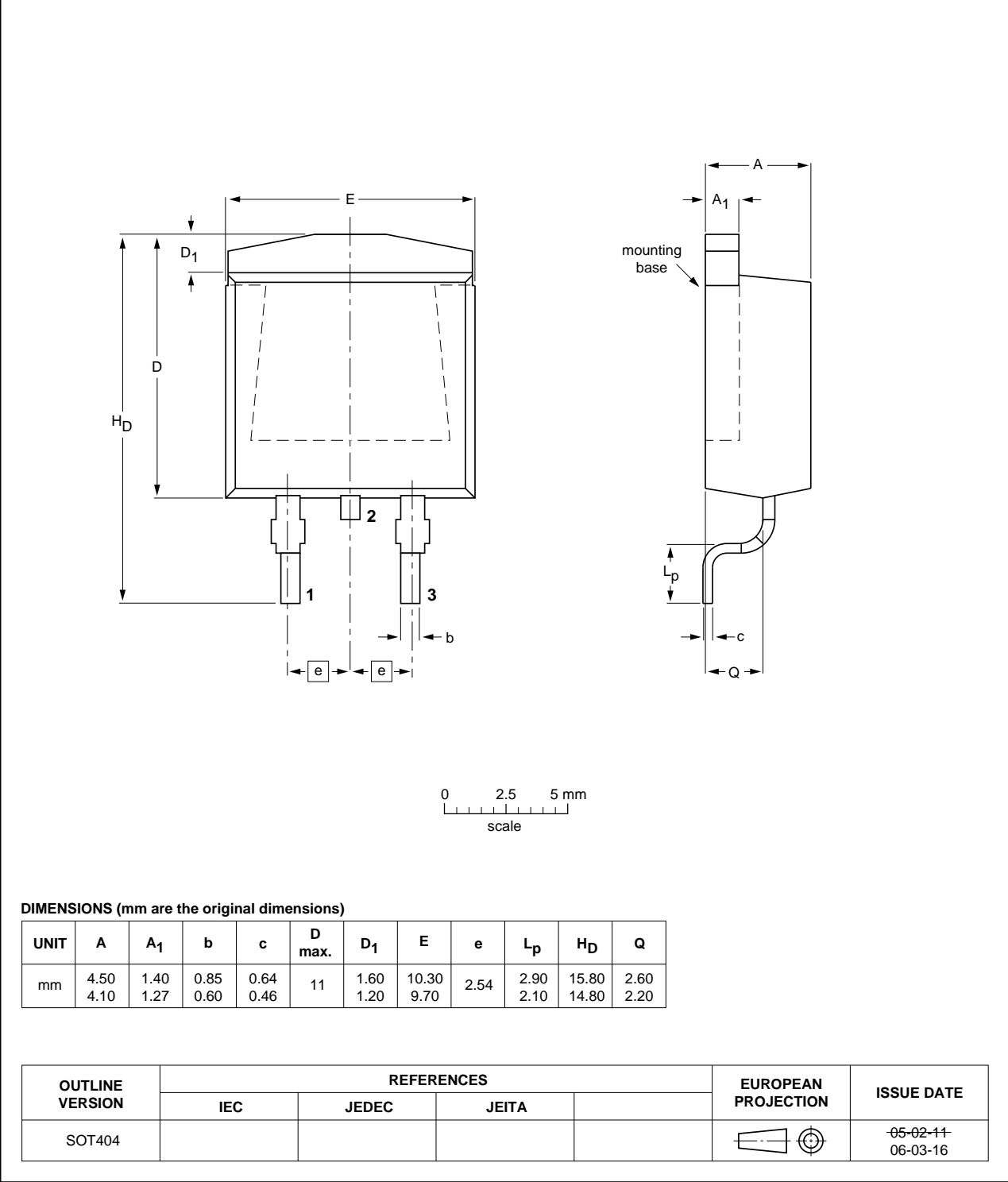
Fig 9. SOT404 (D2PAK).
