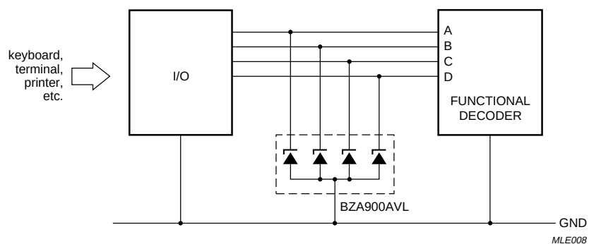
Fig.7 Computer interface protection.
