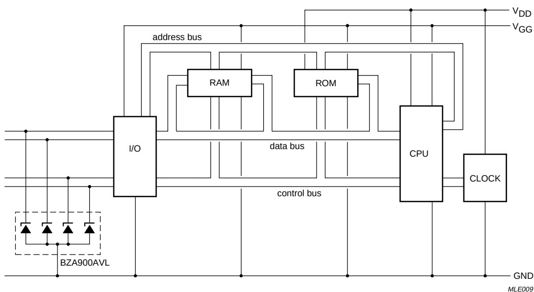
Fig.8 Microprocessor protection.
