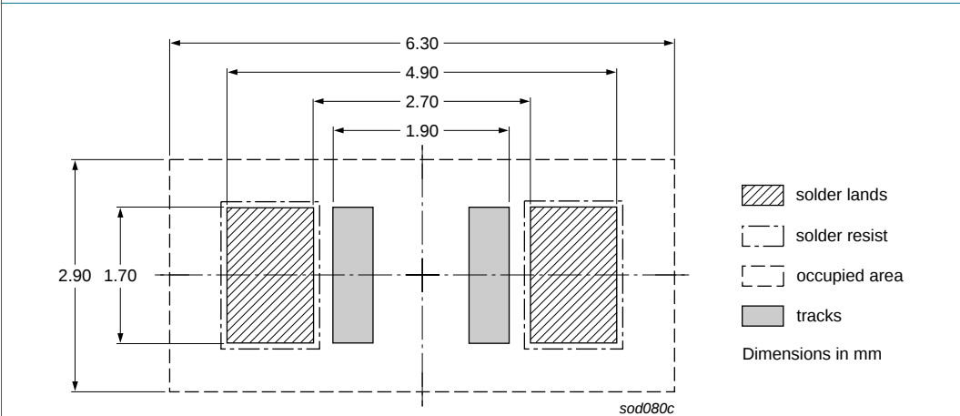
Fig 7. Reflow soldering footprint SOD80C
