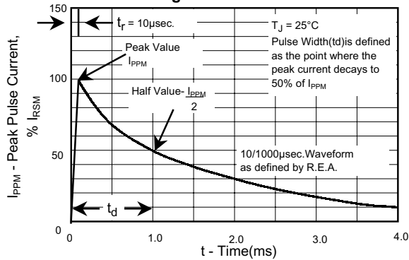
Fig.3 - Pulse Waveform
