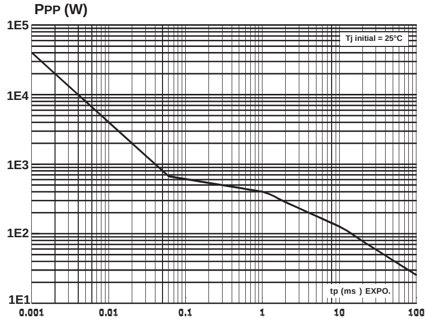
Fig. 2 : Peak pulse power versus exponential pulse duration.
