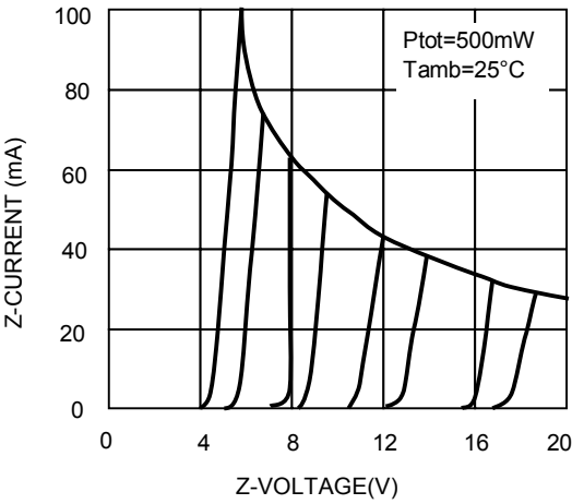
FIG.8 - Z-CURRENT VS. Z-VOLTAGE
